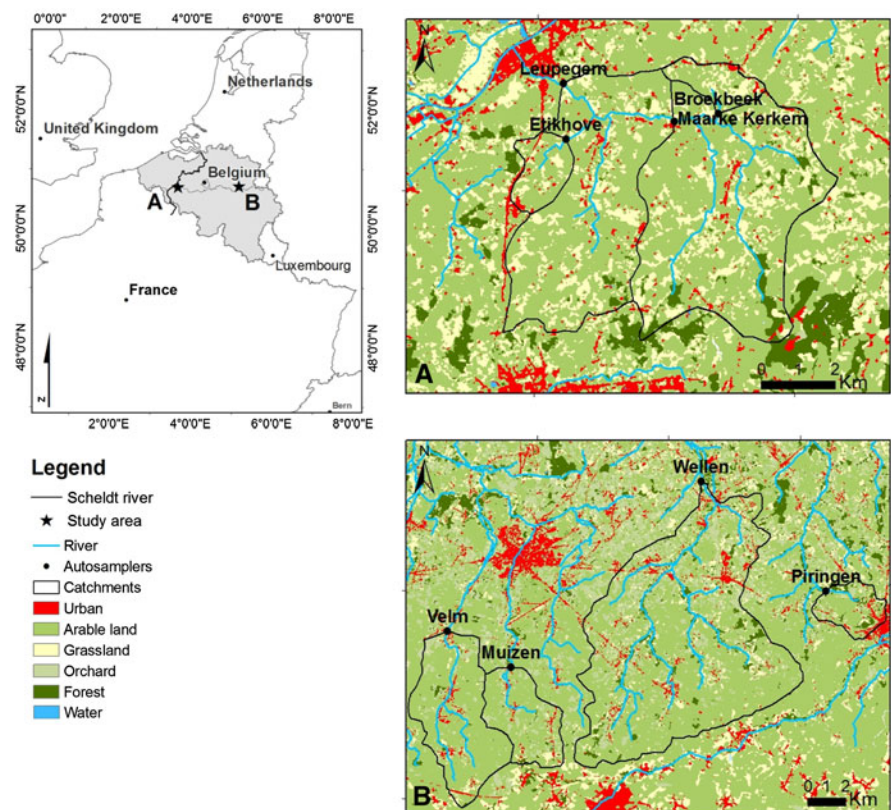
Fig. 1 Map of the location of and land use in the sampled watersheds
