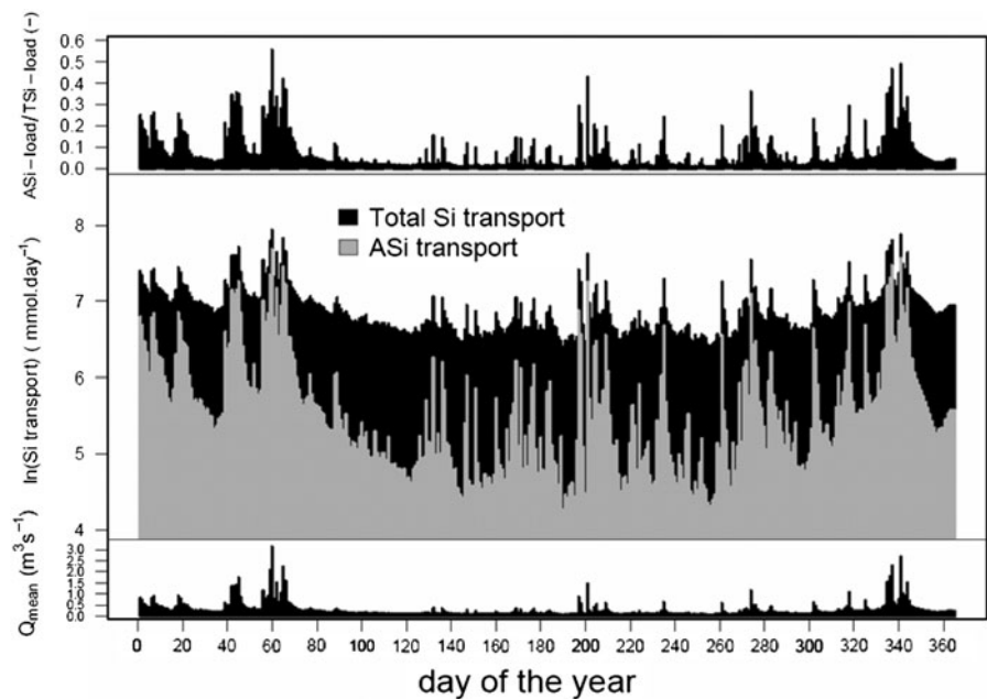
Fig. 6 Time series of discharge, simulated ASi and TSi (ASi + DSi) fluxes and ASi/TSi ratios for the catchment of Leupegem during 2007. Simulated silica loads were calculated following the peak flow scenario “ r = 0.75 ” * and are shown as daily summed values. Q_{\text{mean}} represents the daily averaged discharge. Attention must be paid to the logarithmic (log) scale of each middle graph. * See Table 4
