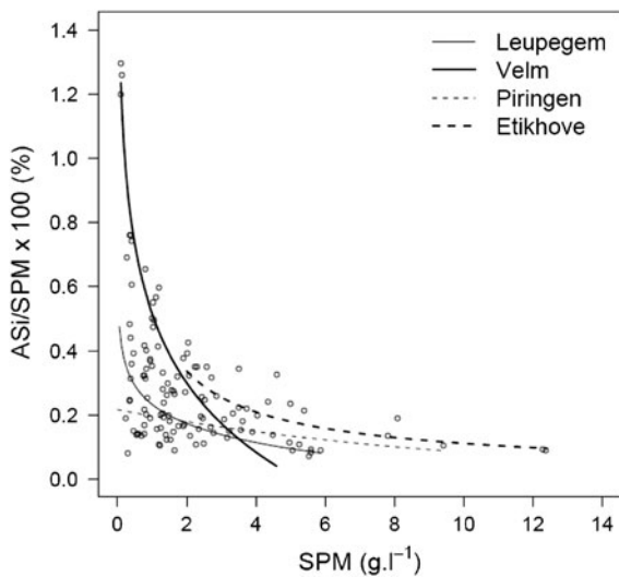
Fig. 4 Decrease in relative amount of amorphous Si (ASi) in suspended matter (SPM) with increasing SPM concentrations, in the four catchments where a significant exponential decrease was observed
