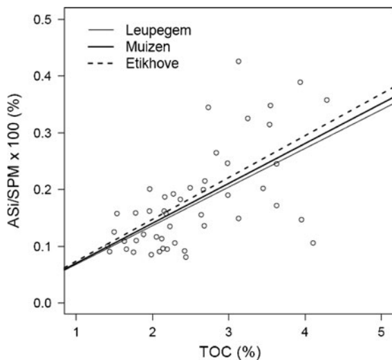
Fig. 5 Relation between total organic carbon (TOC) and amorphous Si (ASi) content in suspended matter (SPM) in the catchments of Leupegem, Muizen and Etikhove. The lines represent the position of the different catchments within the data. All linear regressions were highly significant ( p < 0.0001 ; R^2 > 0.81 )
