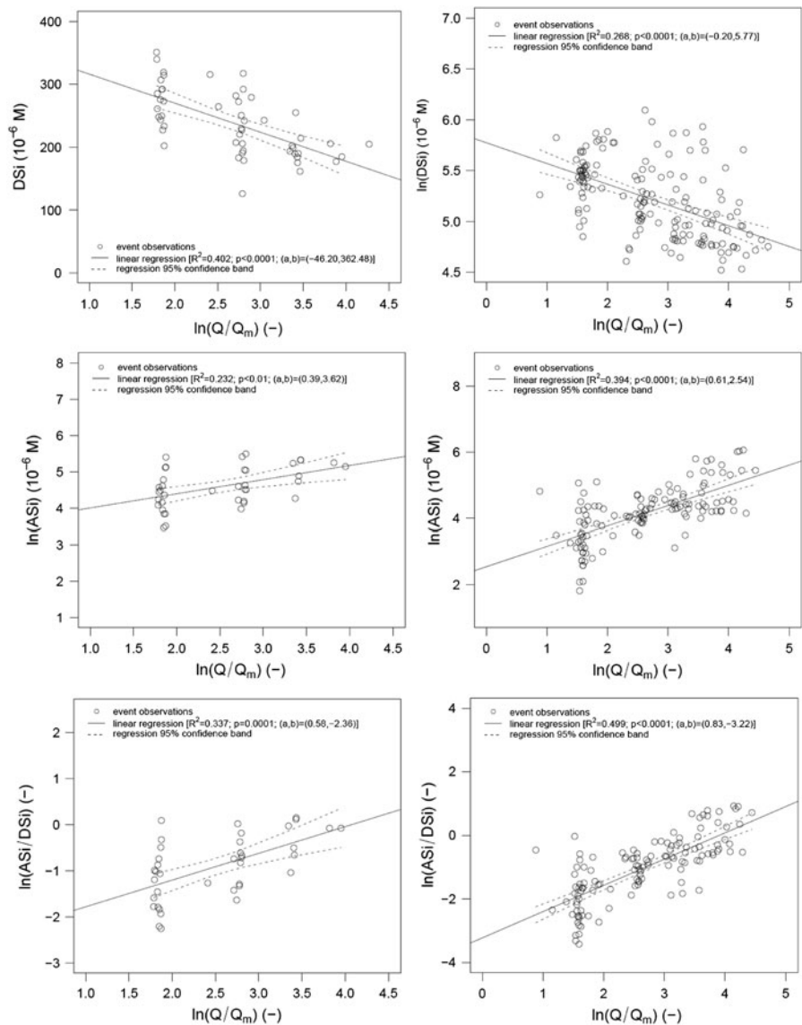
Fig. 3 Relations between relative discharge ( Q/Q_{\text{modal}} ) and DSi and ASi concentrations and relative importance of ASi (ASi/DSi) in the catchments of Leupegem ( left ) and Muizen ( right ). Q_{\text{modal}} is modal discharge from 2006 to 2008
