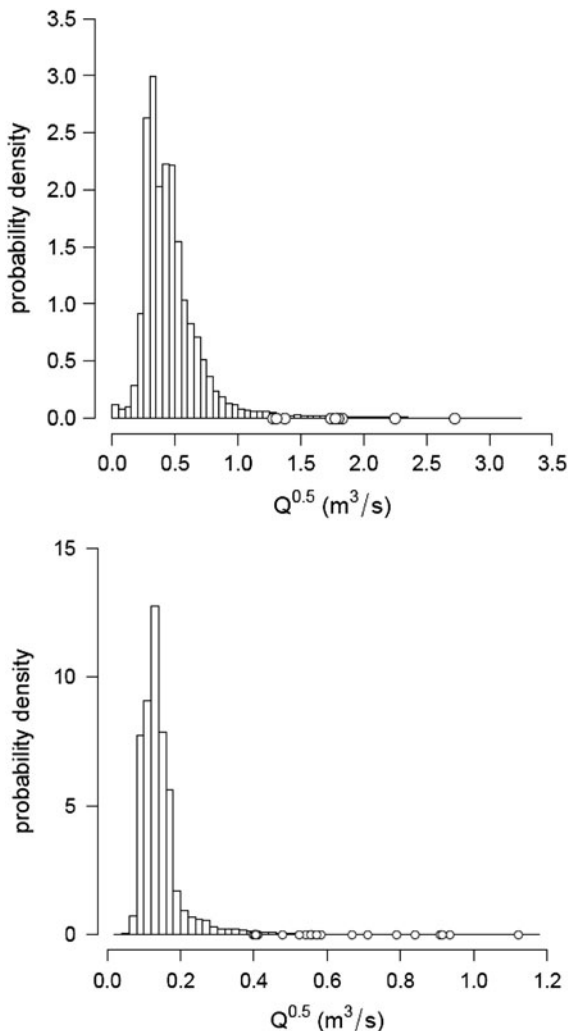
Fig. 2 Discharge distribution in the catchments of Leupegem ( top ) and Muizen ( down ) during the period 2006–2008. All other sampled catchments had similarly skewed distributions. The maximal discharge observed during the sampled peak events is indicated as open white dots on the high discharge end of the distribution
